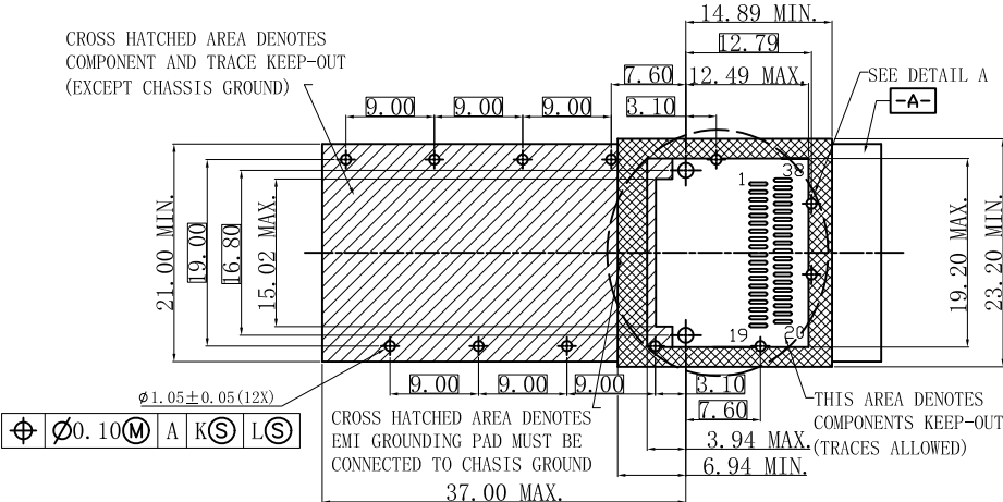
RECOMMENDED HOST PCB BOARD SINGLE SIDE LAYOUT COMPONENT SIDE OF BOARD
